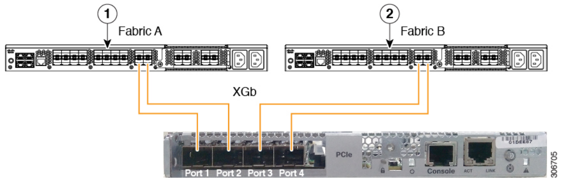
Figure 2: Direct Connect Cabling Configuration with Cisco VIC 1455
