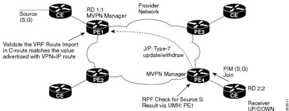
Figure 1: RFC 4761 NLRI
