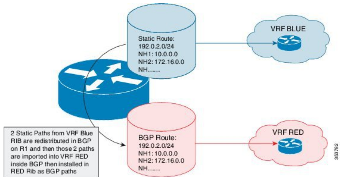
Figure 1: Deployment Scenario for BGP Multiple Paths Replication
