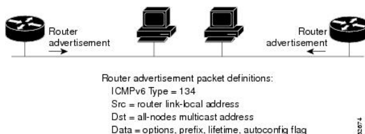
Figure 3: IPv6 Neighbor Discovery--RA Message
