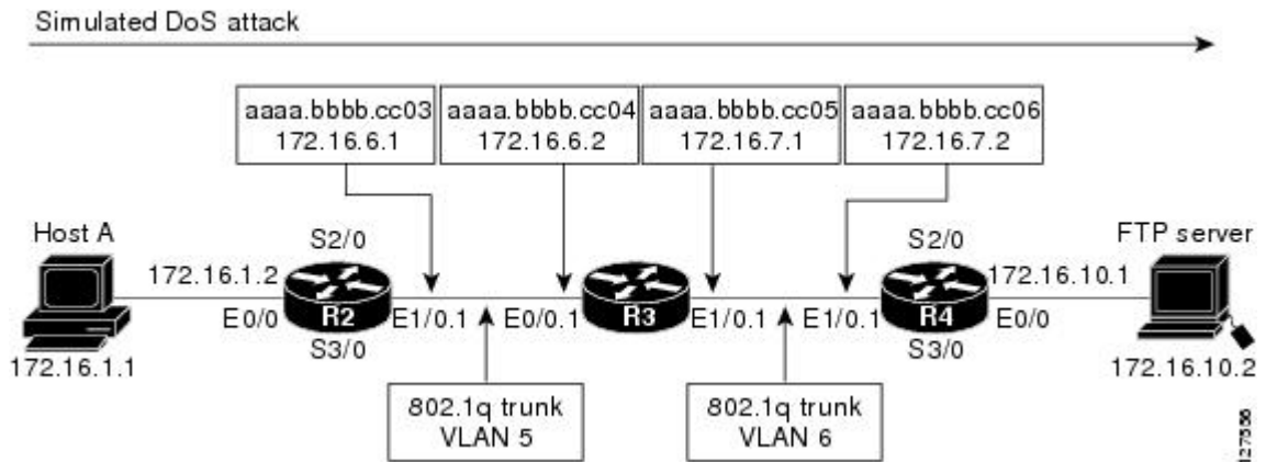
Figure 1 Simulated DoS Attack (b)
