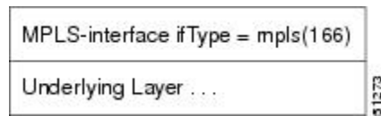
Figure 3: Interface Group MIB Stack Table for MPLS Interfaces
