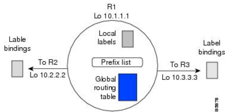
Figure 3: LDP Local Label Allocation Filtering Example
