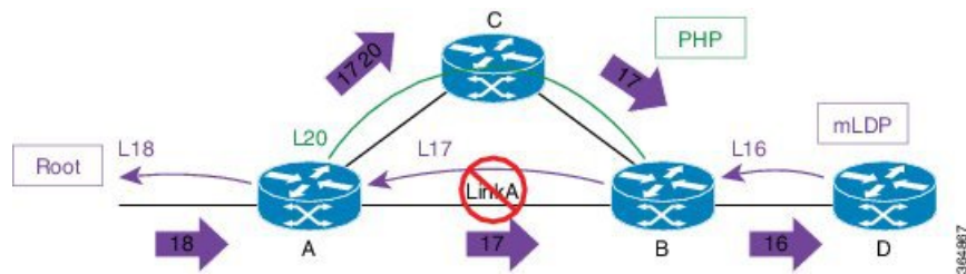
Figure 9: Link Failure
