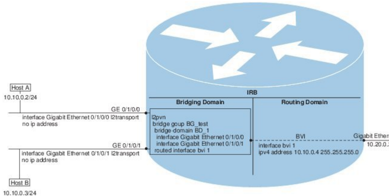
Figure 11: IRB Functional View and Configuration Elements
