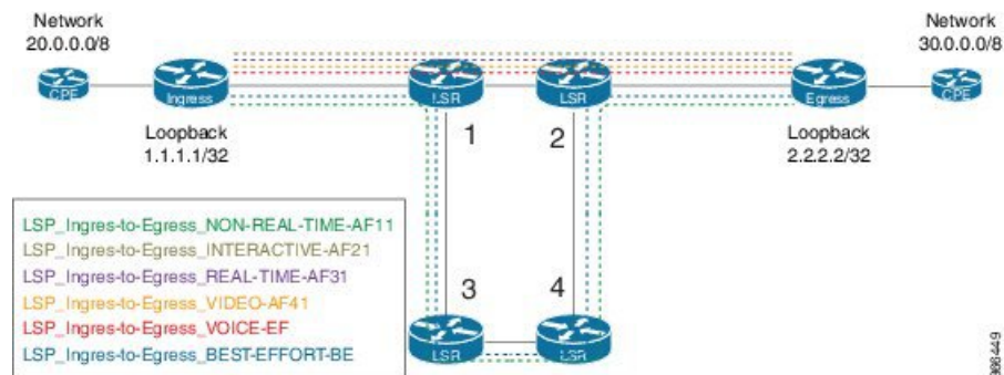
Figure 7: Policy-Based Tunnel Selection Implementation
