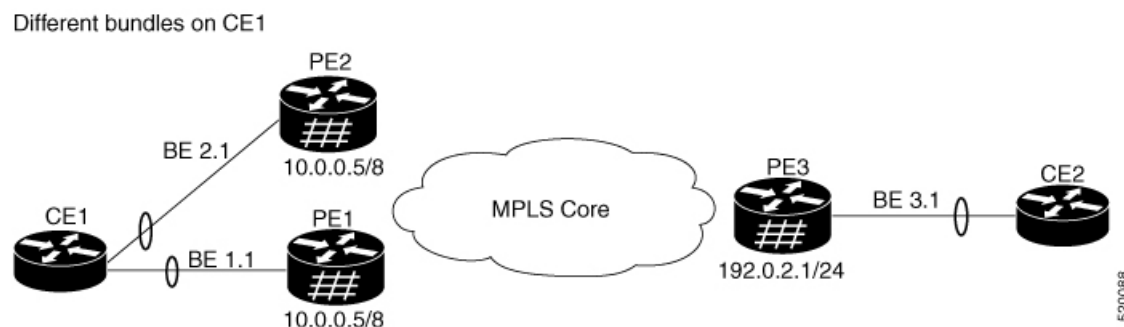
Figure 11: EVPN: Single-Active Multihoming for Anycast Gateway IRB
