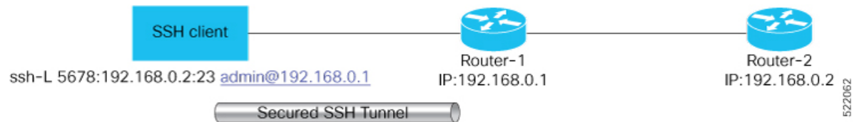
Figure 3: Sample Topology for SSH Port Forwarding
