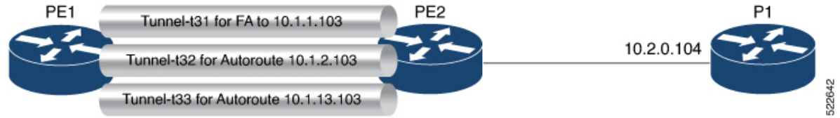
Figure 3: Topology
