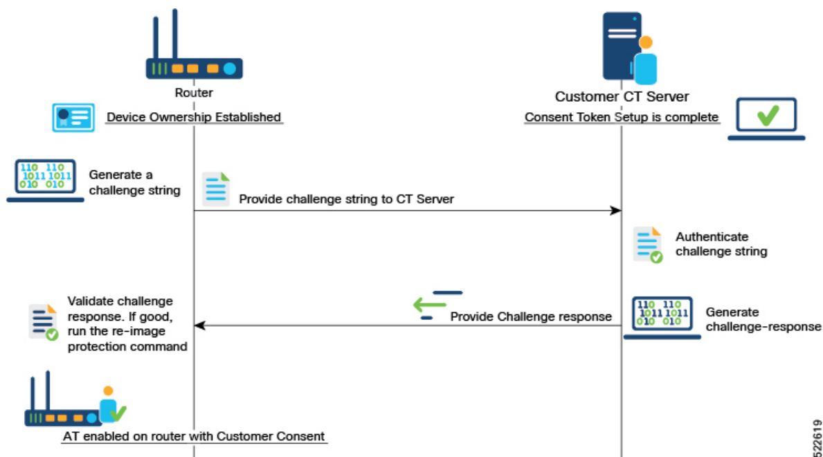
Figure 14: Workflow for the Customer Consent Token Key
