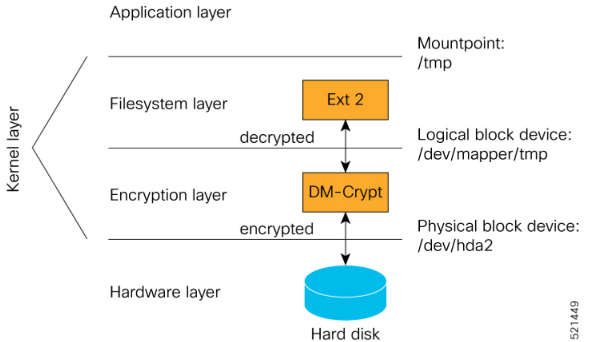
Figure 18: DM-Crypt Encryption
