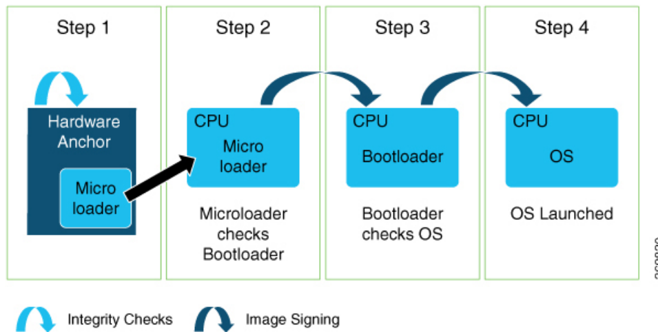
Figure 17: Secure Boot
