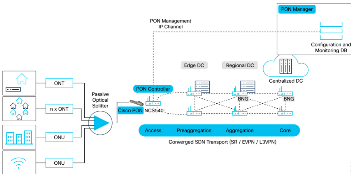
Figure 1: Cisco Routed PON Architecture
