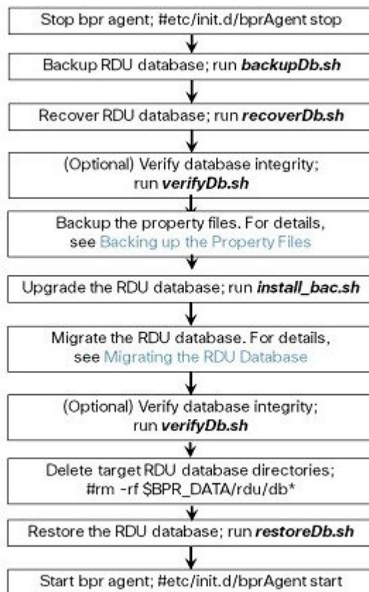
Figure 1: Database Migration
