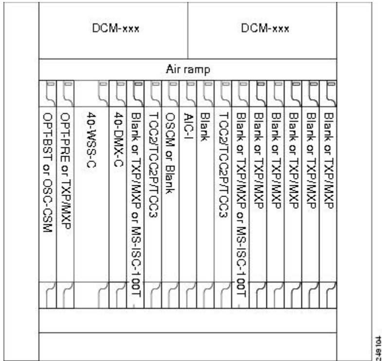
Figure 2: Terminal Node Configuration with 40-WSS-C Cards Installed
