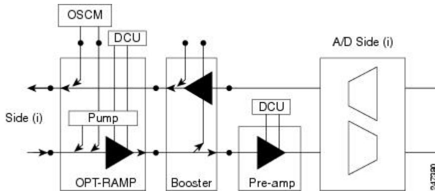
Figure 69: OPT-RAMP-C or OPT-RAMP-CE Card in an Add/Drop Node
