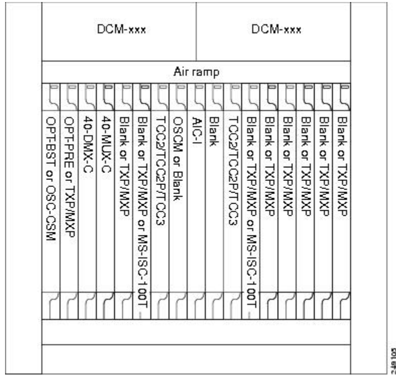
Figure 3: Terminal Node with 40-MUX-C Cards Installed
