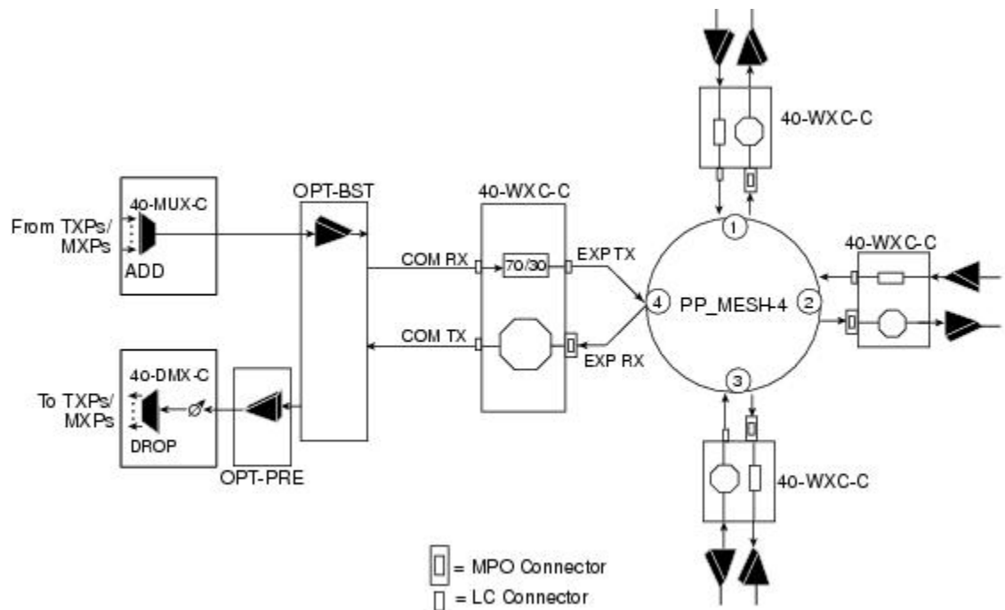
Figure 102: Mesh Node With Omni-Directional Add/Drop Section
