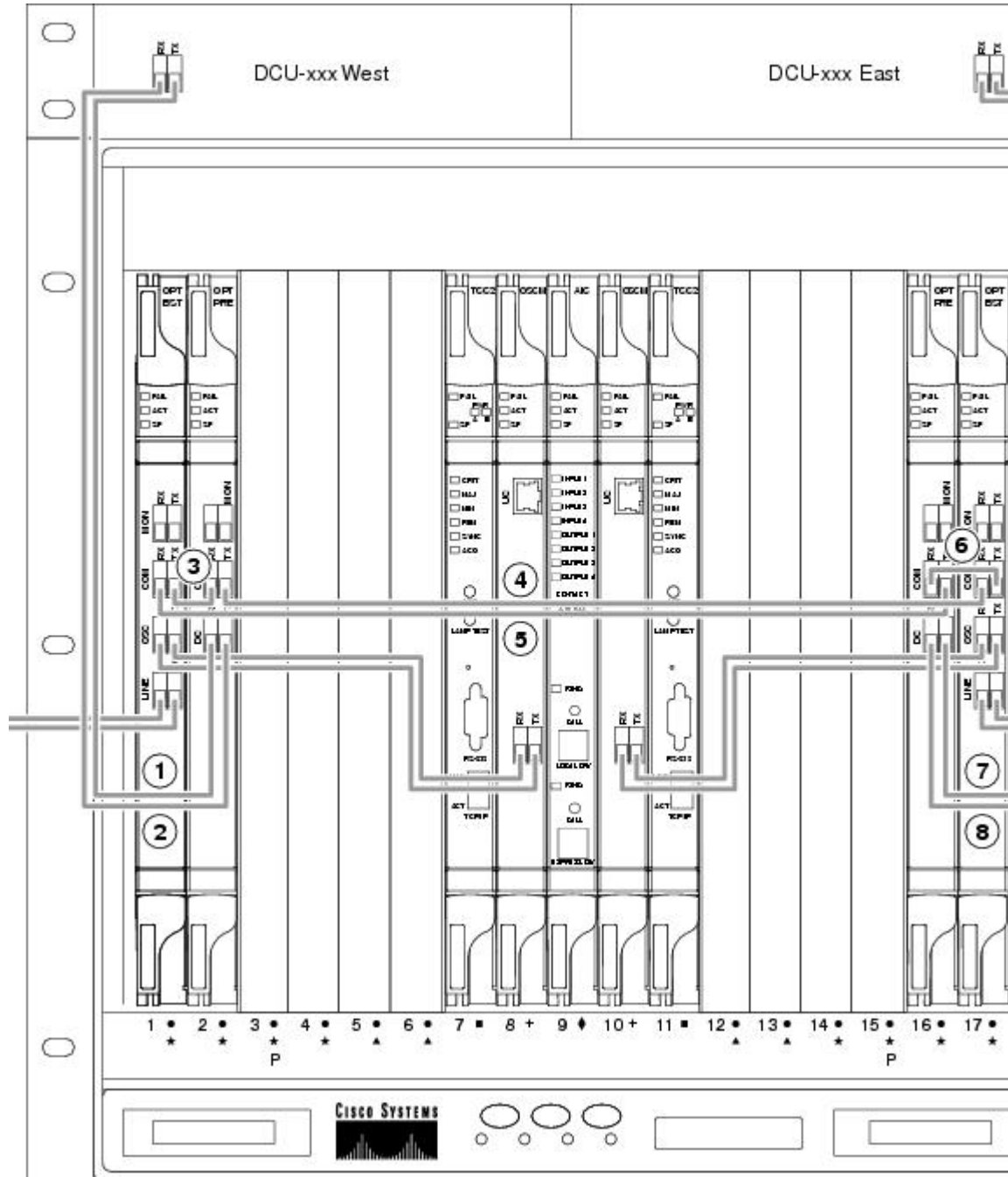
Figure 105: Fiberizing a Line Amplifier Node
