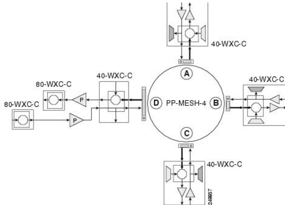
Figure 88: 40-Channel Colorless and Omni-directional Four-Degree ROADM Node
