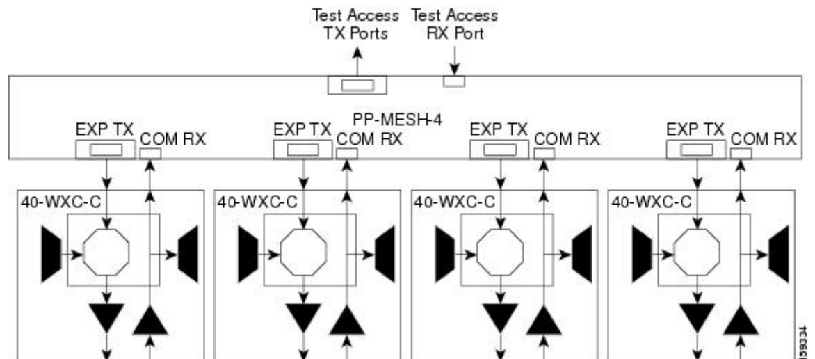
Figure 99: PP-MESH-4 Patch Panel Signal Flow
