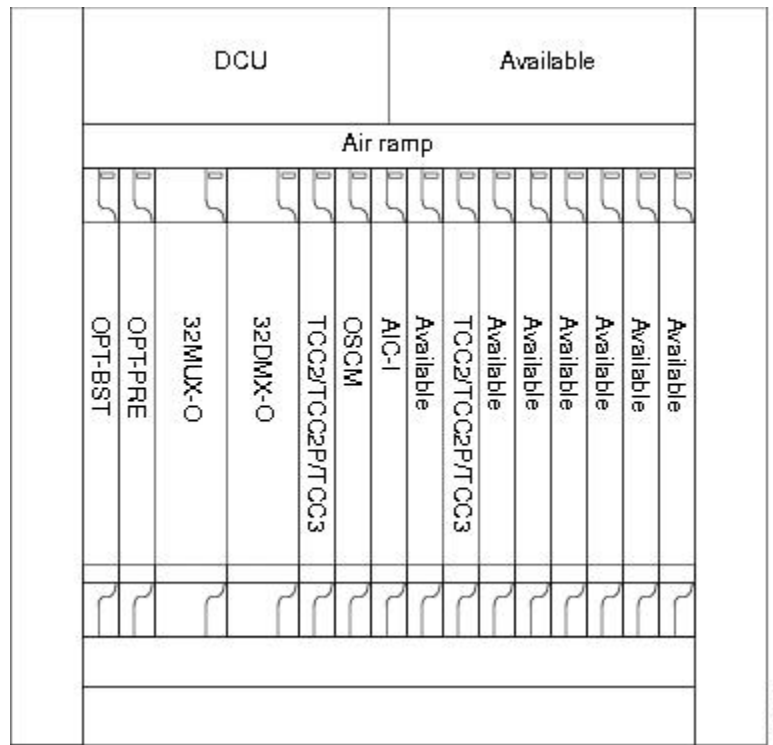
Figure 1: Terminal Node Configuration With 32MUX-O Cards Installed
