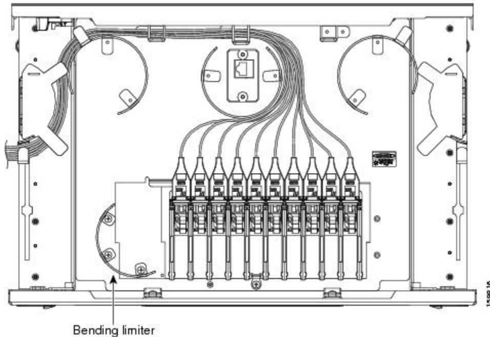
Figure 11: 40-Channel Patch Panel Tray, Top View
