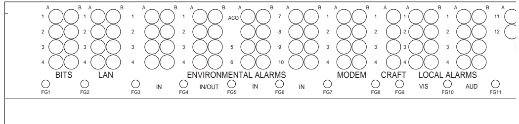
Figure 1-28 ONS 15454 Backplane Pinouts (Release 3.4 or Higher)
