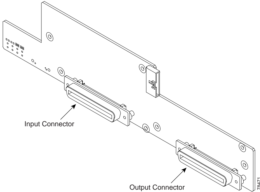
Figure 1-22 AEP Printed Circuit Board Assembly
