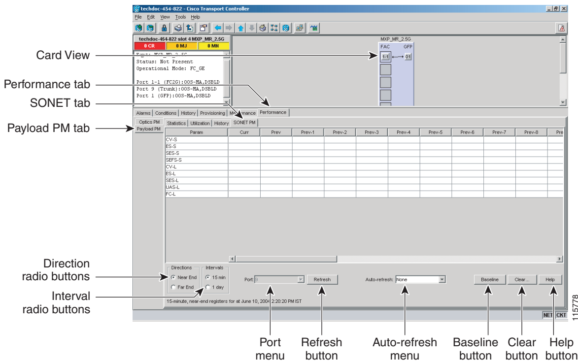
Figure 8-13 SONET PM Tab on the Card View Performance Window
