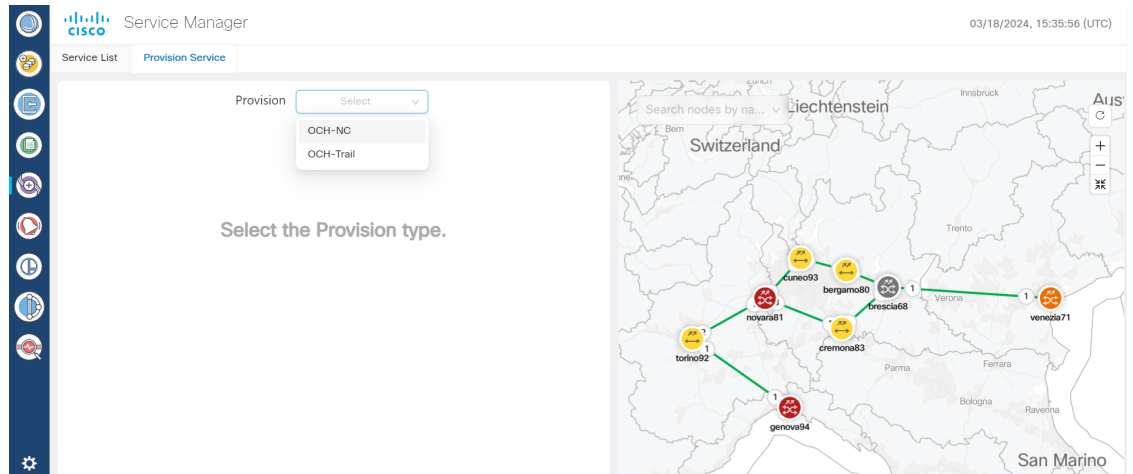
Figure 11: Provision Service
