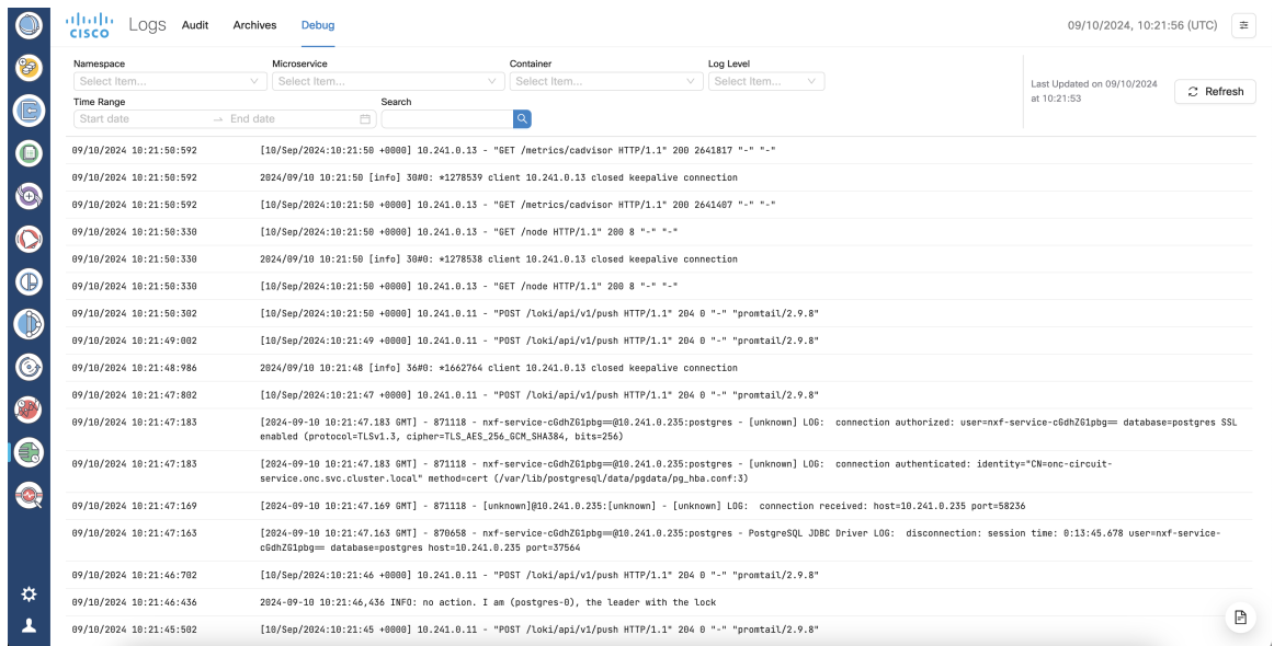
Figure 27: Debug Logs
