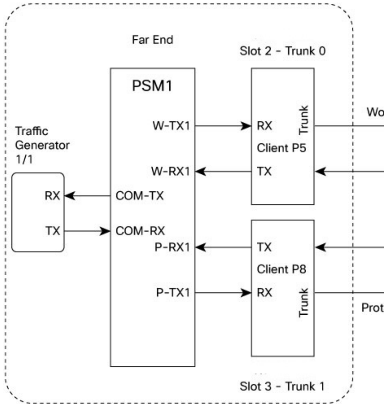
Figure 3: Reference Topology for Protection Switching
