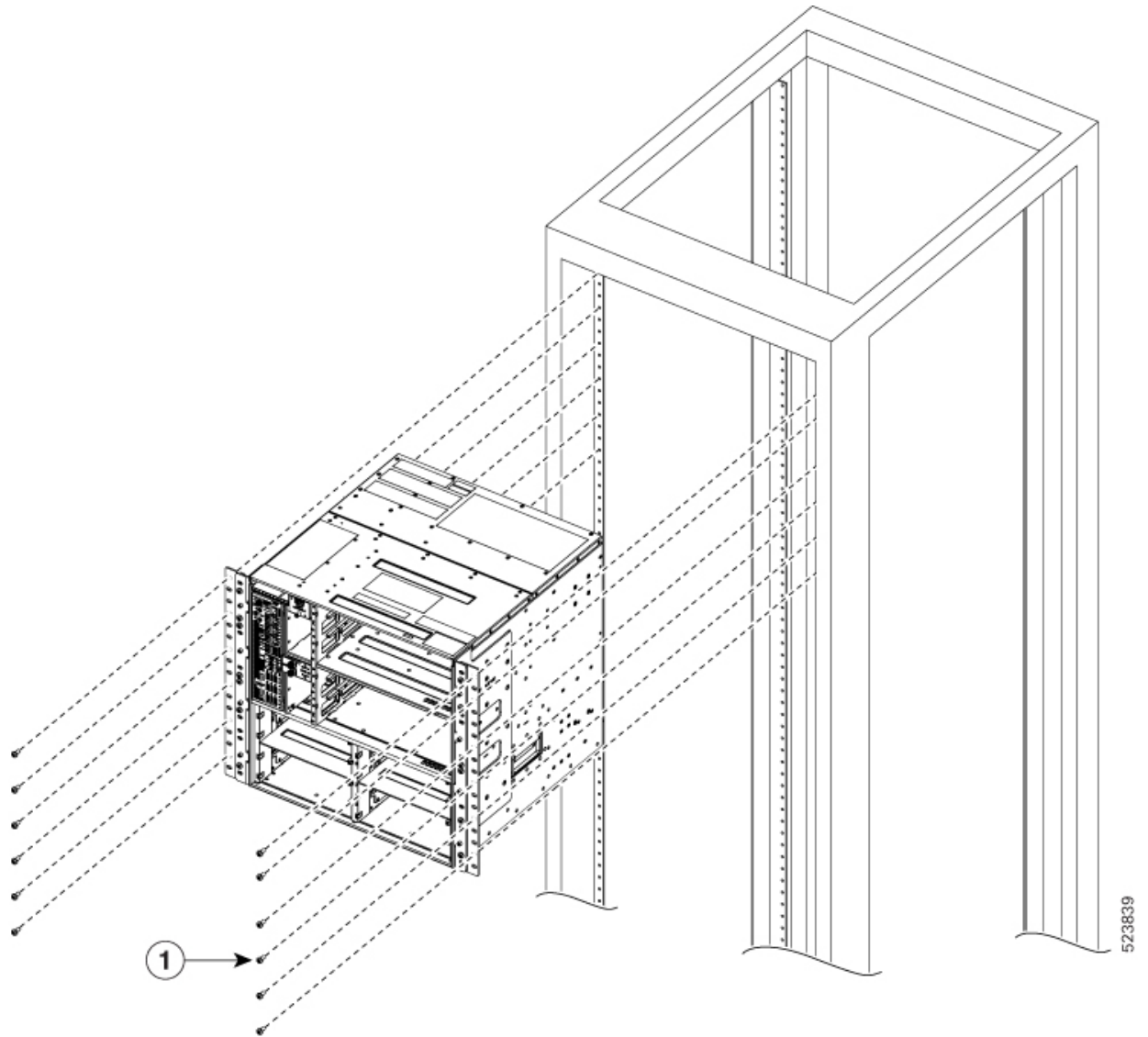
Figure 7: Mounting the NCS 1020 on a Four-Post ETSI Rack
