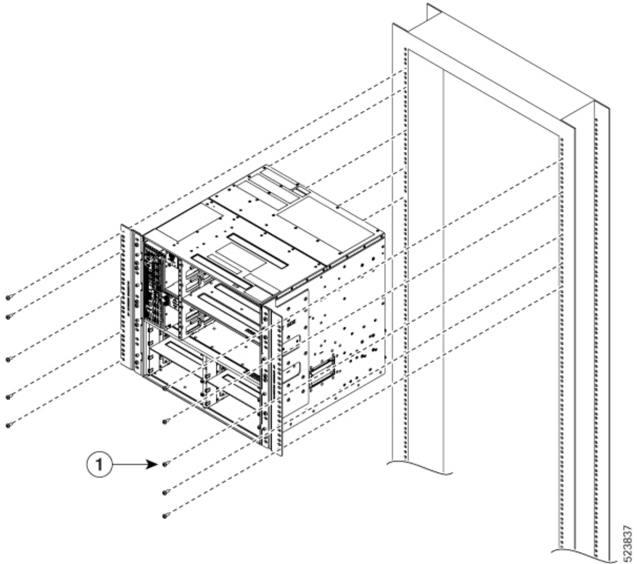
Figure 8: Mounting the NCS 1020 on a Two-Post ANSI Rack
