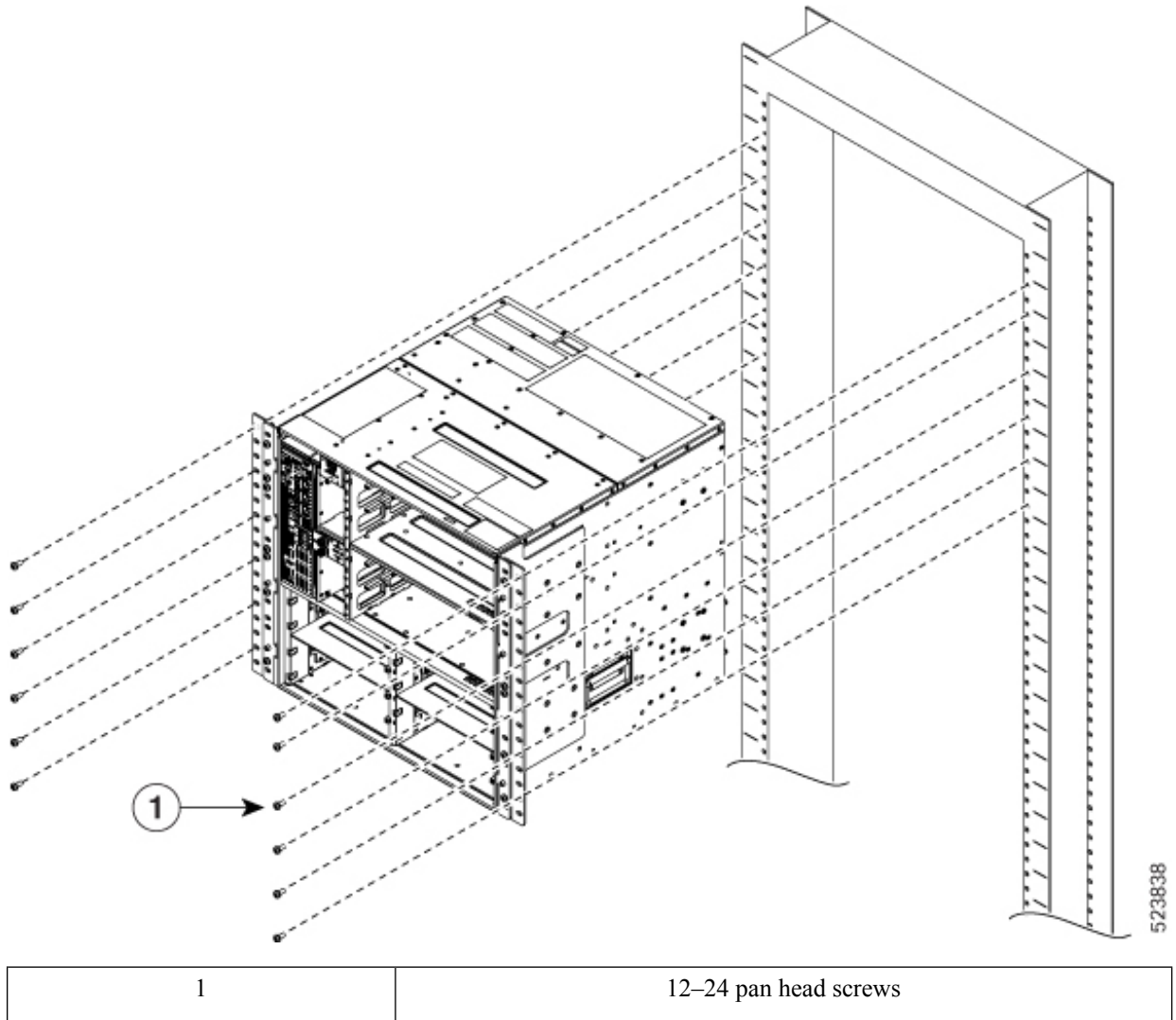
Figure 6: Mounting the NCS 1020 on a Two-Post ETSI Rack
