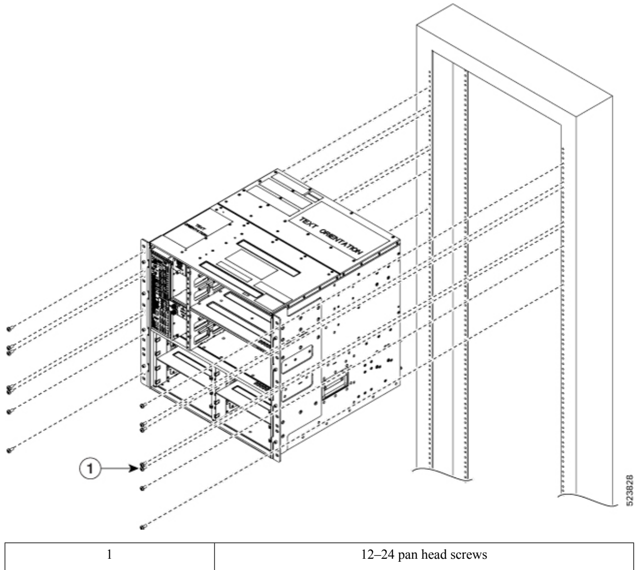
Figure 4: Mounting the NCS 1020 on a Two-Post 19" Rack
