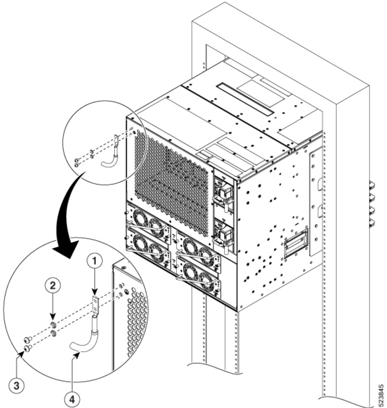
Figure 10: NCS 1020 Ground Lug
