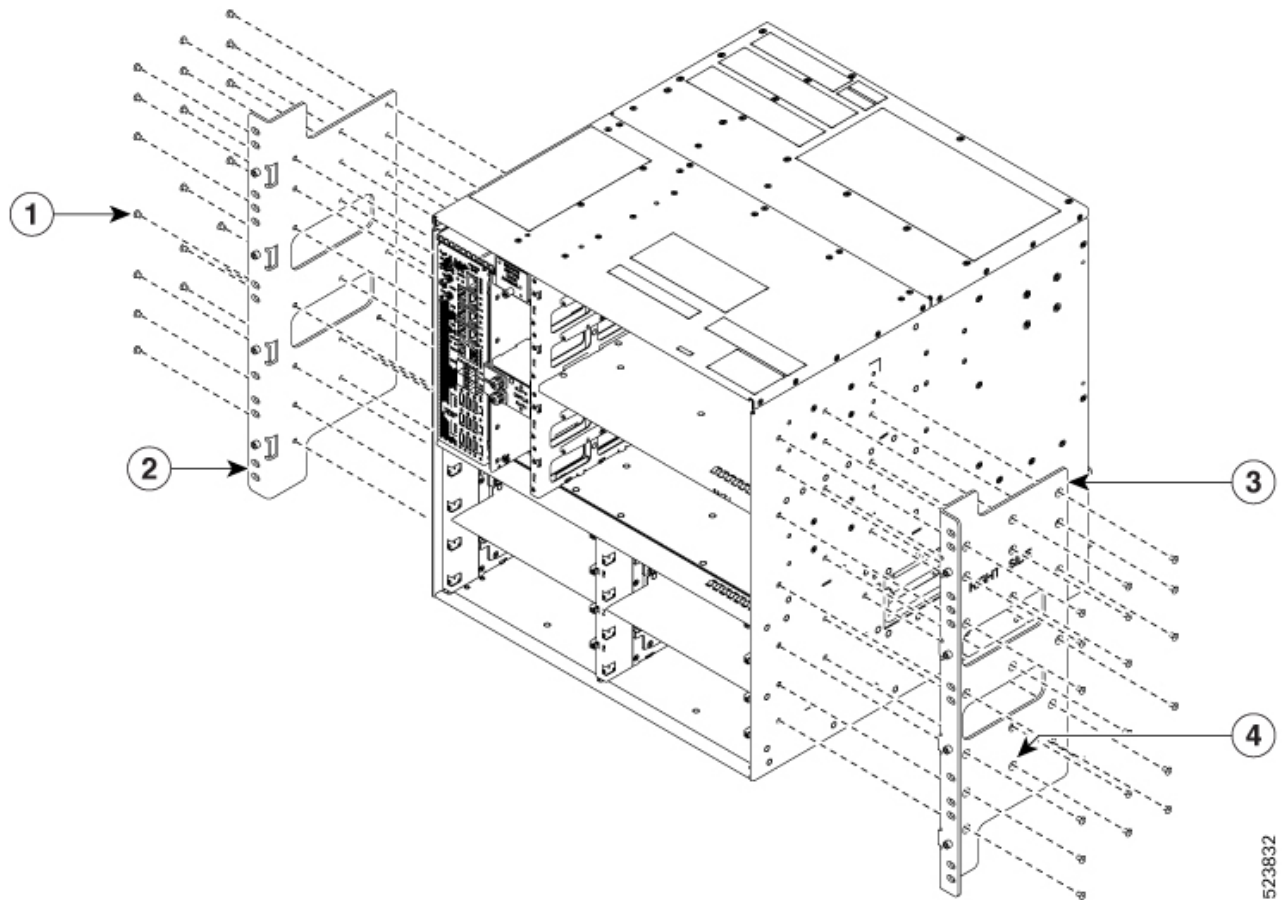
Figure 3: Attaching the Mounting Brackets on an Empty Chassis
