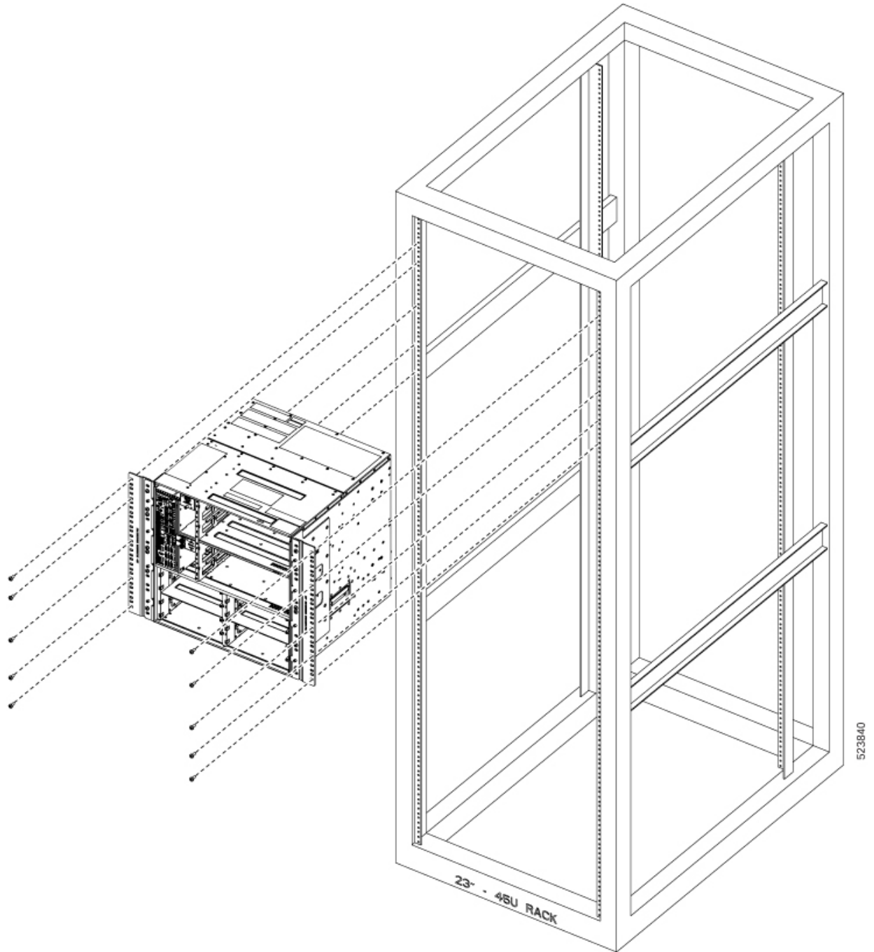
Figure 9: Mounting the NCS 1020 on a Four-Post ANSI Rack
