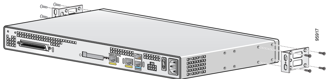
Figure 3-4 Telco 19-Inch Rack Installation—Rear Panel Forward
