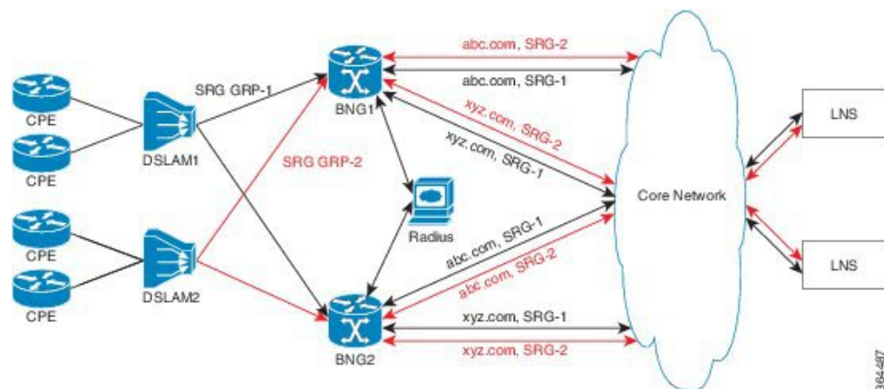
Figure 30: PPPoE-LAC Geo Redundancy Topology
