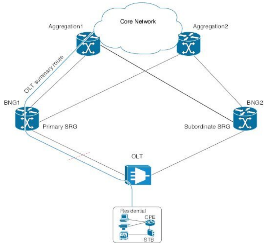
Figure 34: State Control Route for BNG Geo Redundancy
