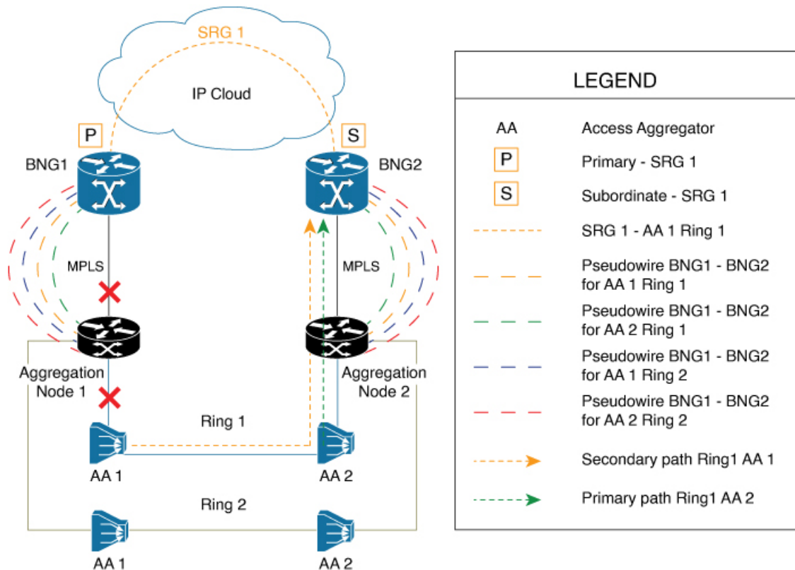
Figure 37: Link Failure Scenarios in BNG PWHE topology with SRG
