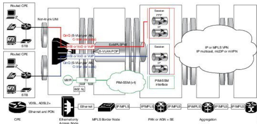
Figure 45: 1:1 deployment model for residential subscribers on PWHE
