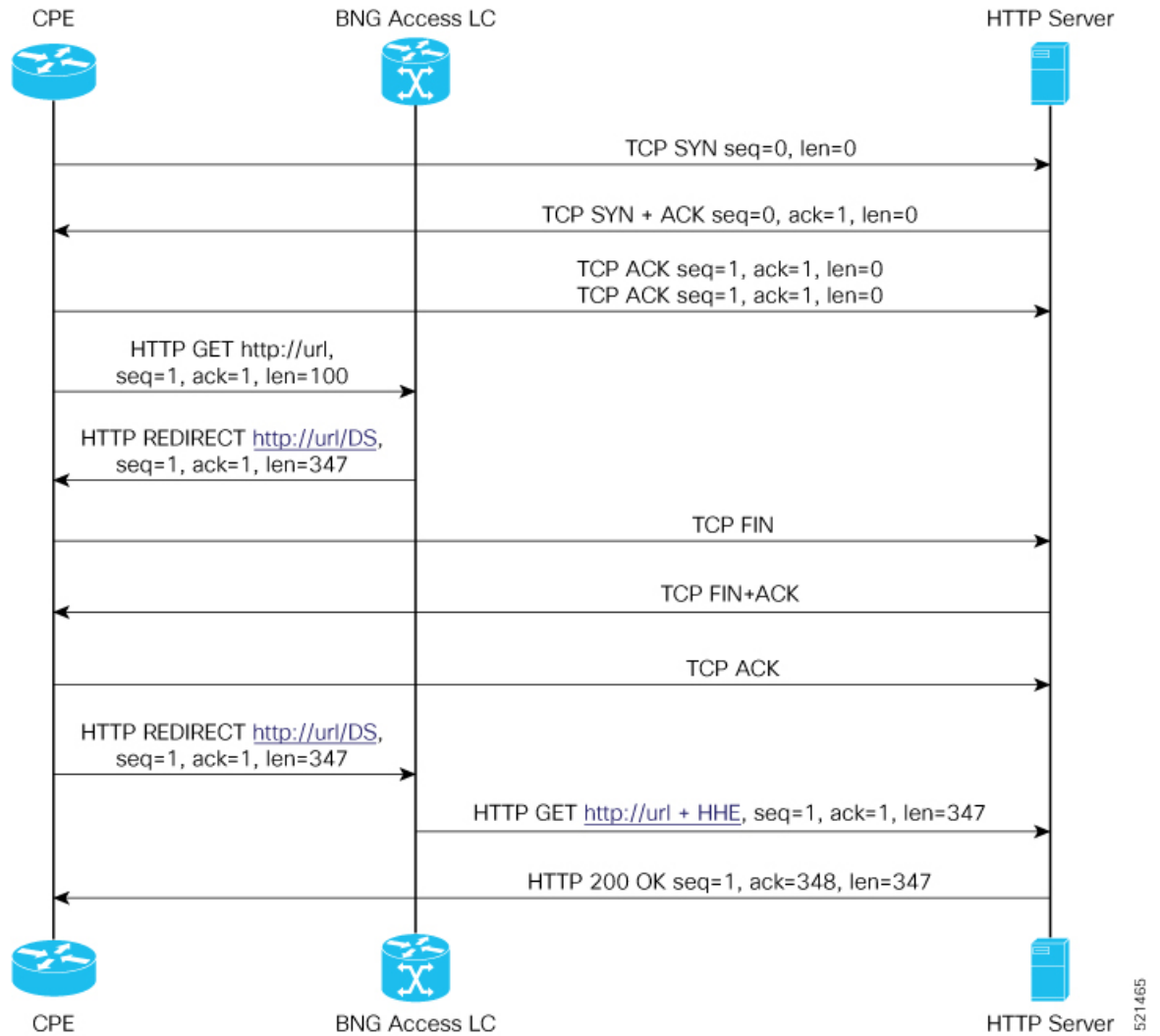
Figure 3: Sequence of events for HTTP Header Enrichment
