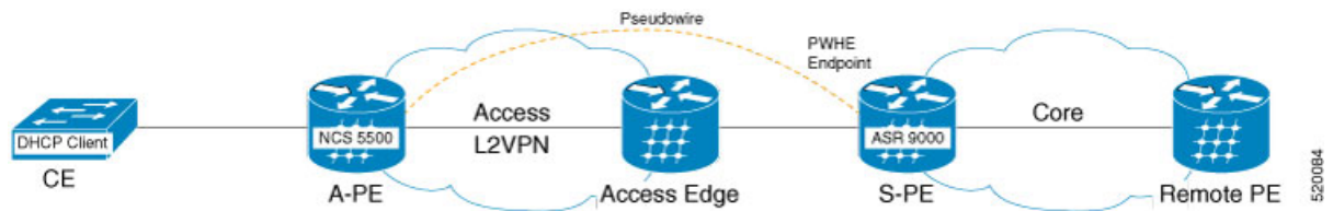
Figure 14: DHCP Functionality for PWHE Interfaces
