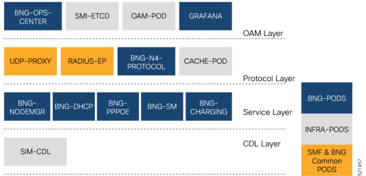
Figure 3: cnBNG Cluster Pod Layout
