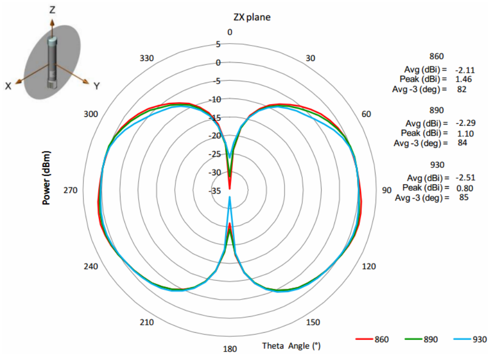
Figure 13-2 Radiation Pattern — Vertical Plane
