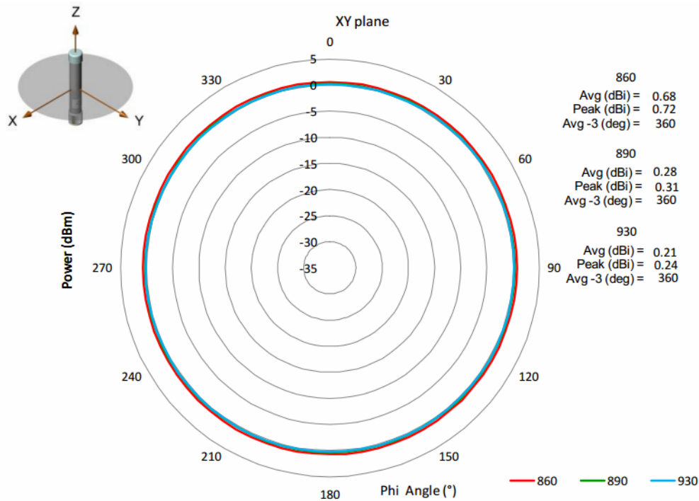
Figure 13-3 Radiation Pattern — Horizontal Plane
