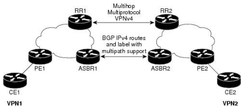
Figure 9: VPNs Using eBGP and iBGP to Distribute Routes and MPLS Labels
