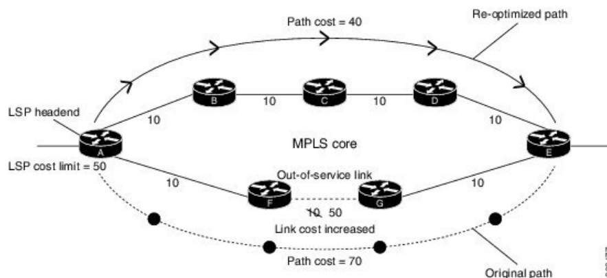
Figure 22: MPLS TE path cost limit application
