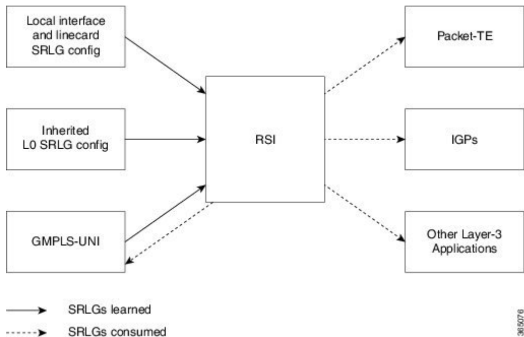
Figure 26: SRLG Communication
