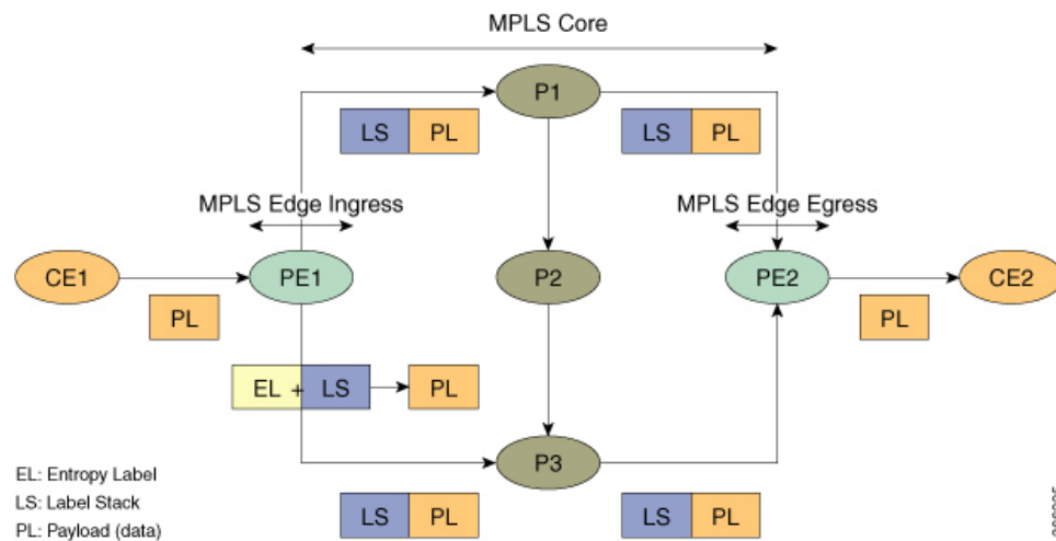
Figure 25: Transit of an MPLS Packet with an Entropy Label
