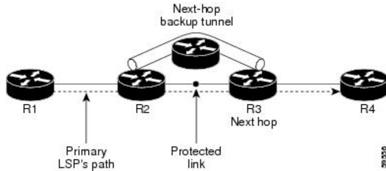
Figure 12: Link Protection
