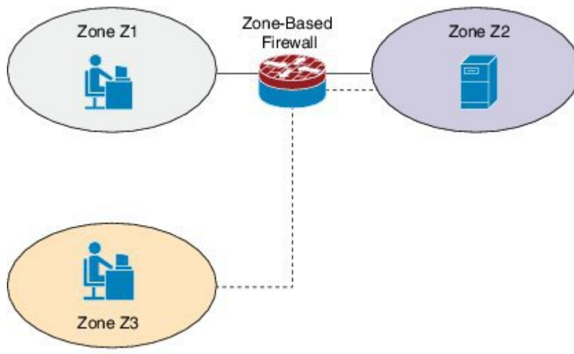
Figure 1: Traffic Inspection by the Zone-Based Firewall
