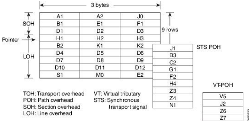
Figure 5: STS-1 Overhead
