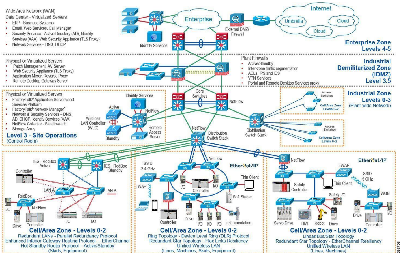
Figure 1-1 CPwE Architectures
