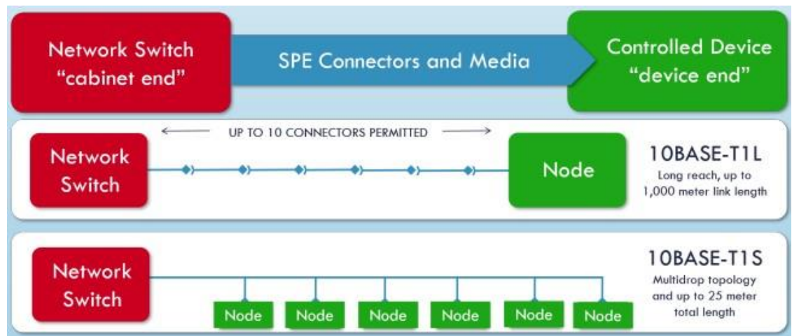
Figure 2-8 Single pair Ethernet architecture
