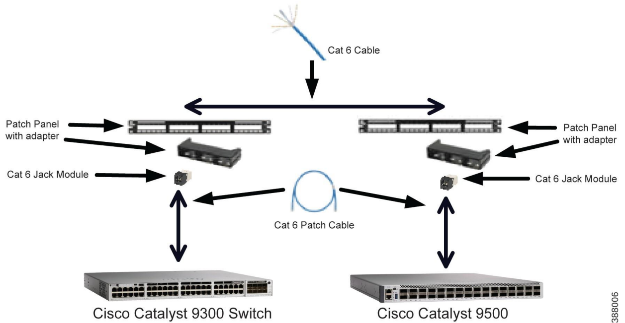
Figure 5-13 Catalyst 9300 Switch to Catalyst 9500 Switch Single Line
