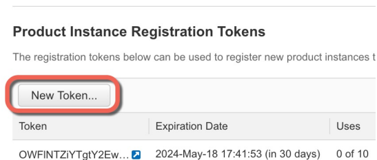
Figure 2: New Token
