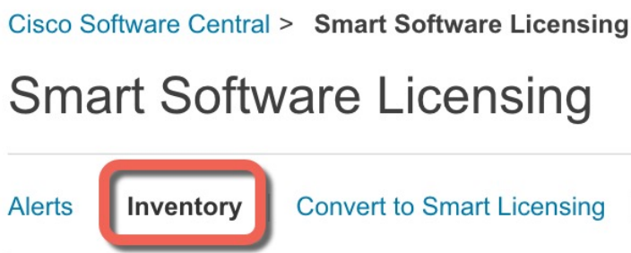
Figure 7: New Token
