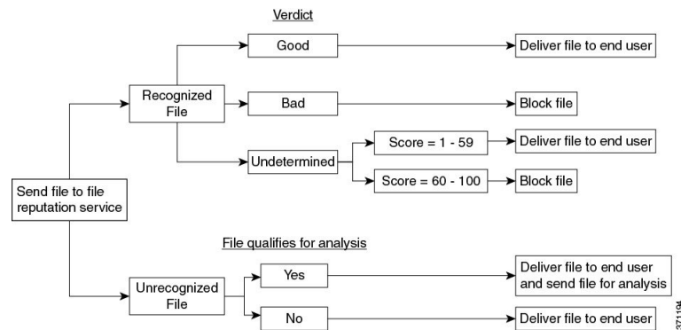
Figure 34: Advanced Malware Protection Workflow for Public-Cloud File Analysis Deployments
