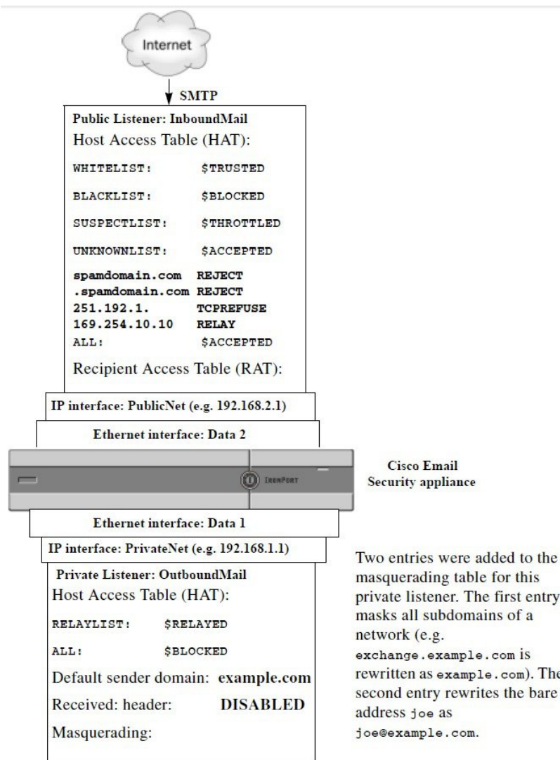
Figure 49: Masquerading Defined for a Private Listener
