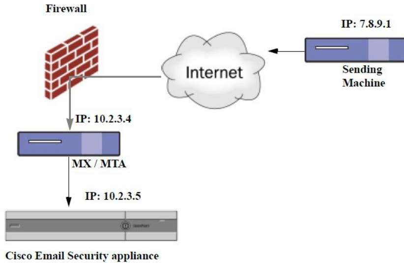
Figure 26: Mail Relayed by MX/MTA — Simple
