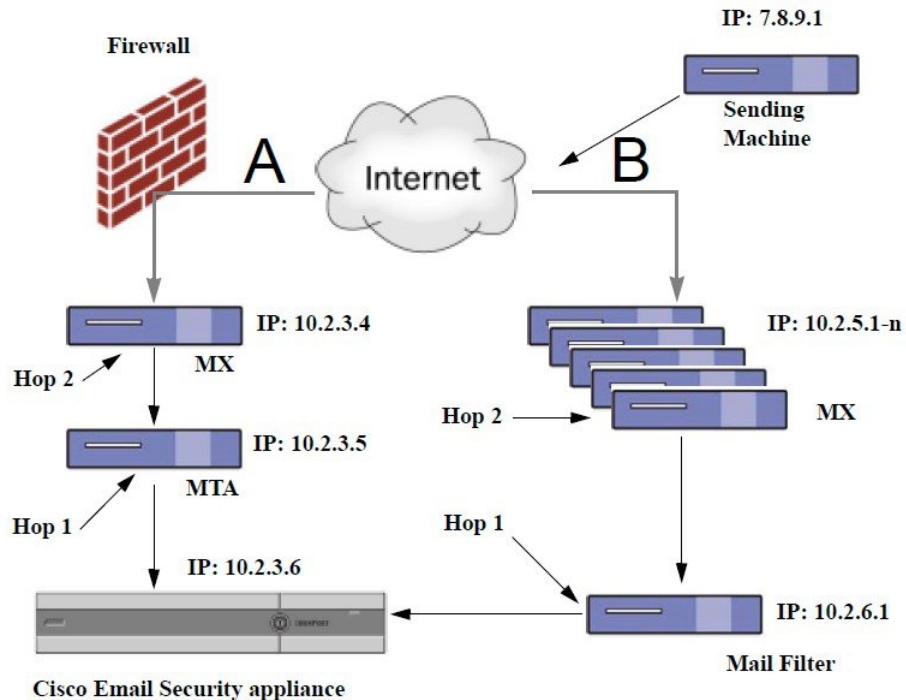
Figure 27: Mail Relayed by MX/MTA — Advanced
