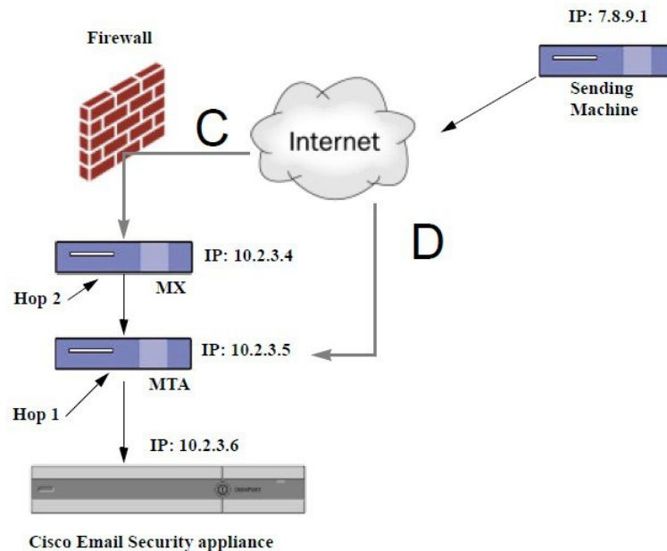
Figure 28: Mail Relayed by MX/MTA — Variable Number of Hops
