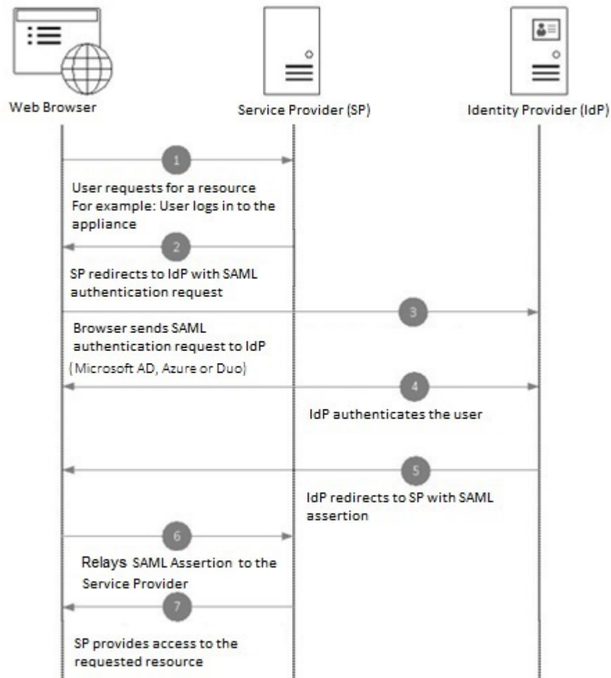
Figure 77: SAML Workflow
