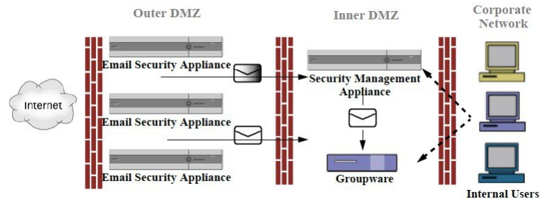
Figure 90: Typical Network Configuration with Cisco Secure Email and Web Manager
