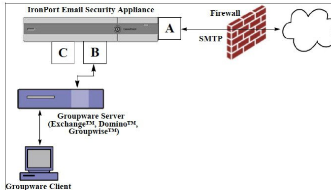
Figure 89: Sinkhole Listener for an Enterprise Gateway
