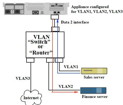
Figure 78: Using VLANs to Facilitate Communication Between Email Gateways
