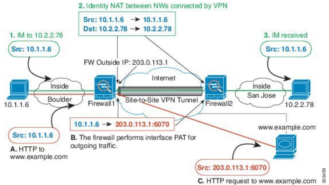
Figure 1: Interface PAT and Identity NAT for Site-to-Site VPN
