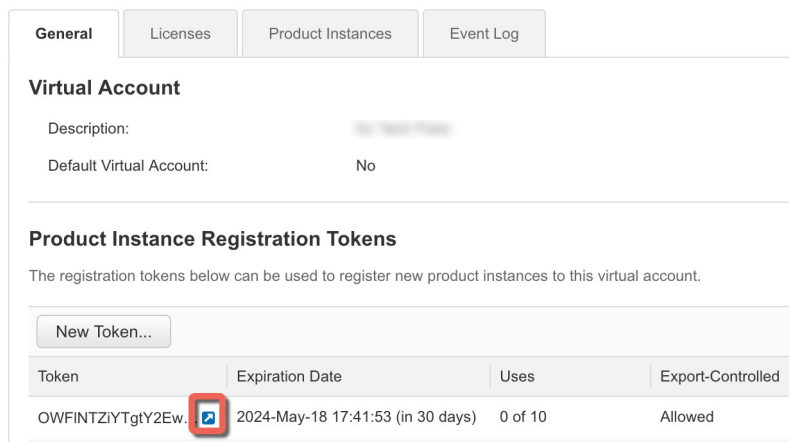
Figure 2: Copy Token
