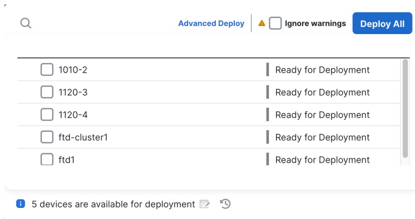
Figure 40: Deploy All
