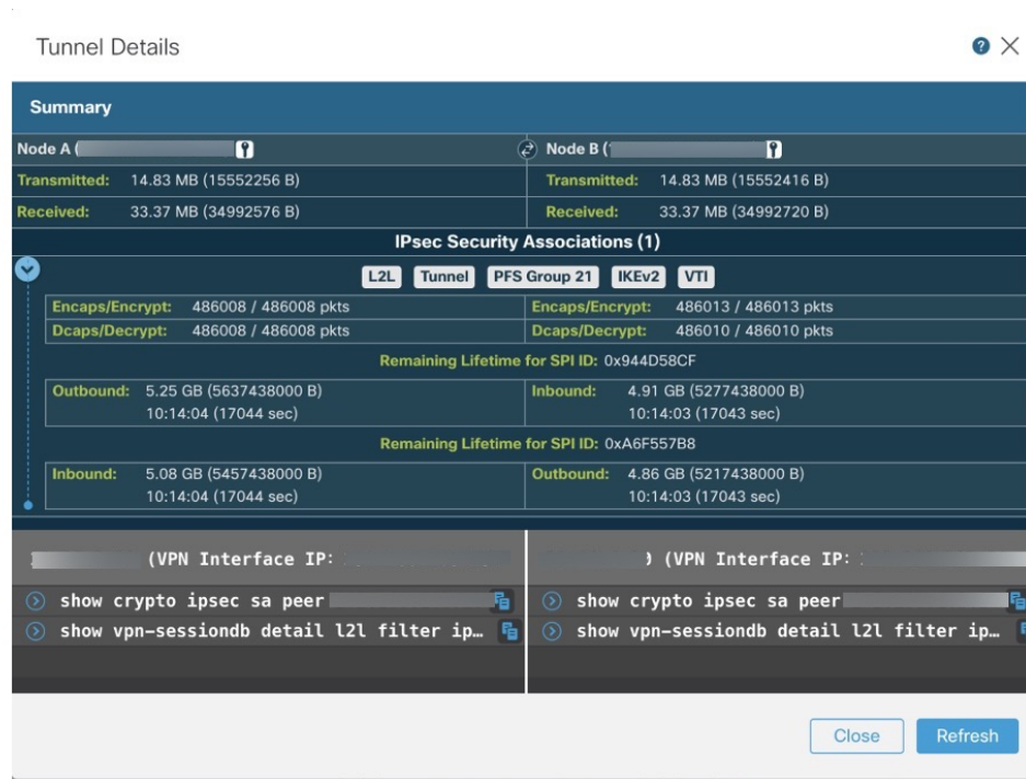
Figure 1: Tunnel Status > View > CLI Details
