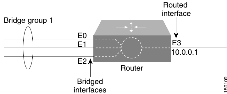
Figure 63-1 Transparent Bridging
