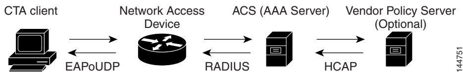
Figure 64-2 NAC System Flow
