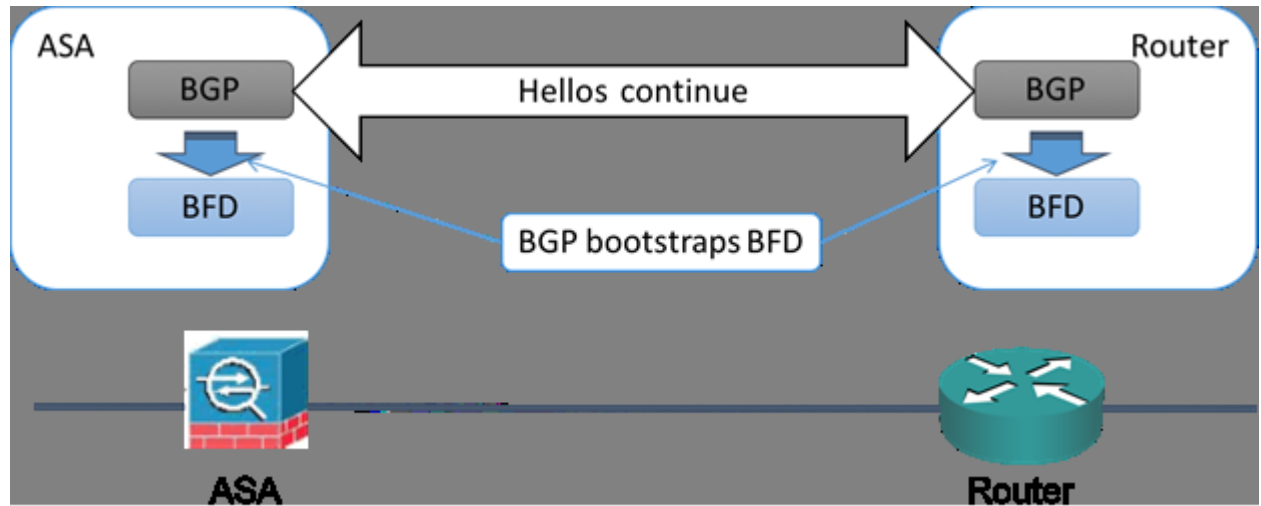
Figure 1: BFD Session Initiated
