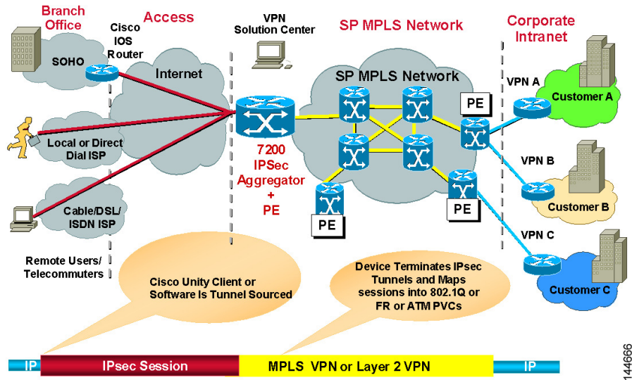
Figure 7: VRF-Aware IPsec One-Box Solution
