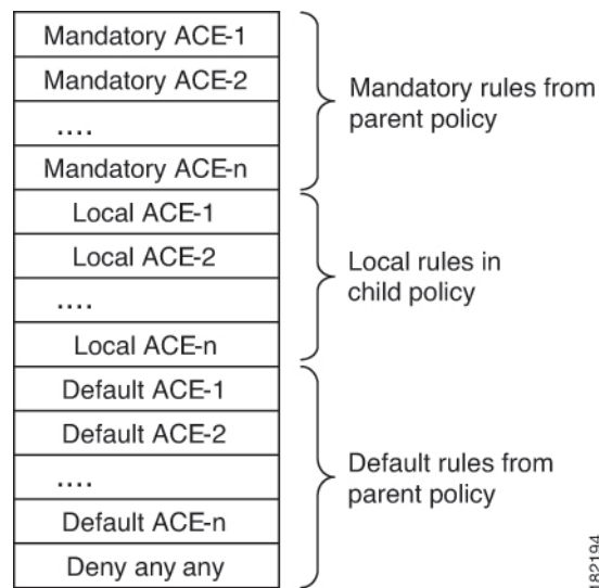
Figure 2: Order of Rules When Using Inheritance
