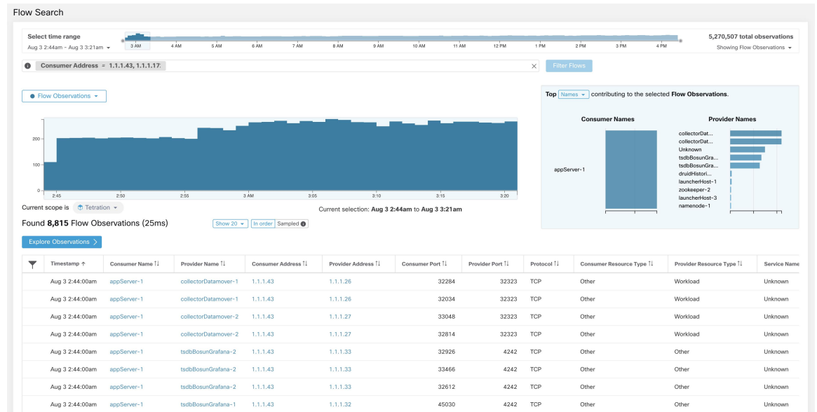
Figure 4: Filter Input Supports for Consumer Address
