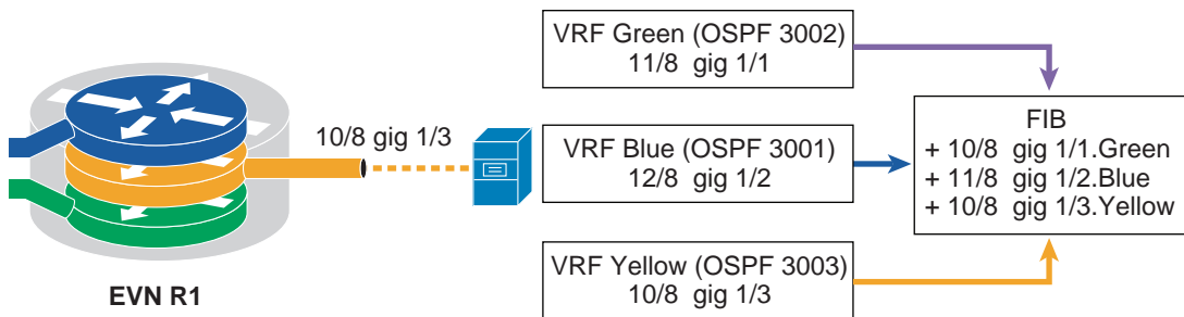
Figure 17 EVN Route Replication
