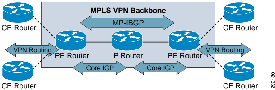
Figure 25 Routing Protocols in MPLS
