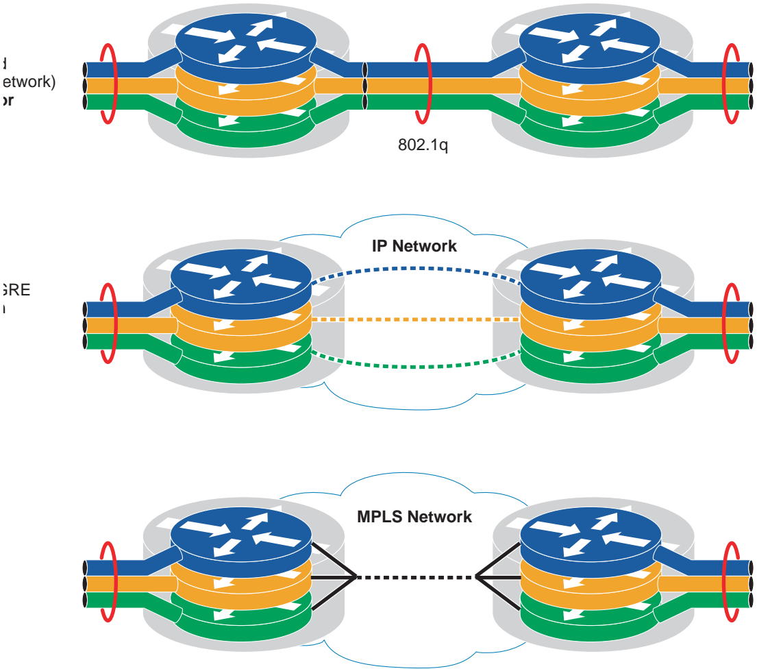
Figure 5 Path Isolation Techniques
