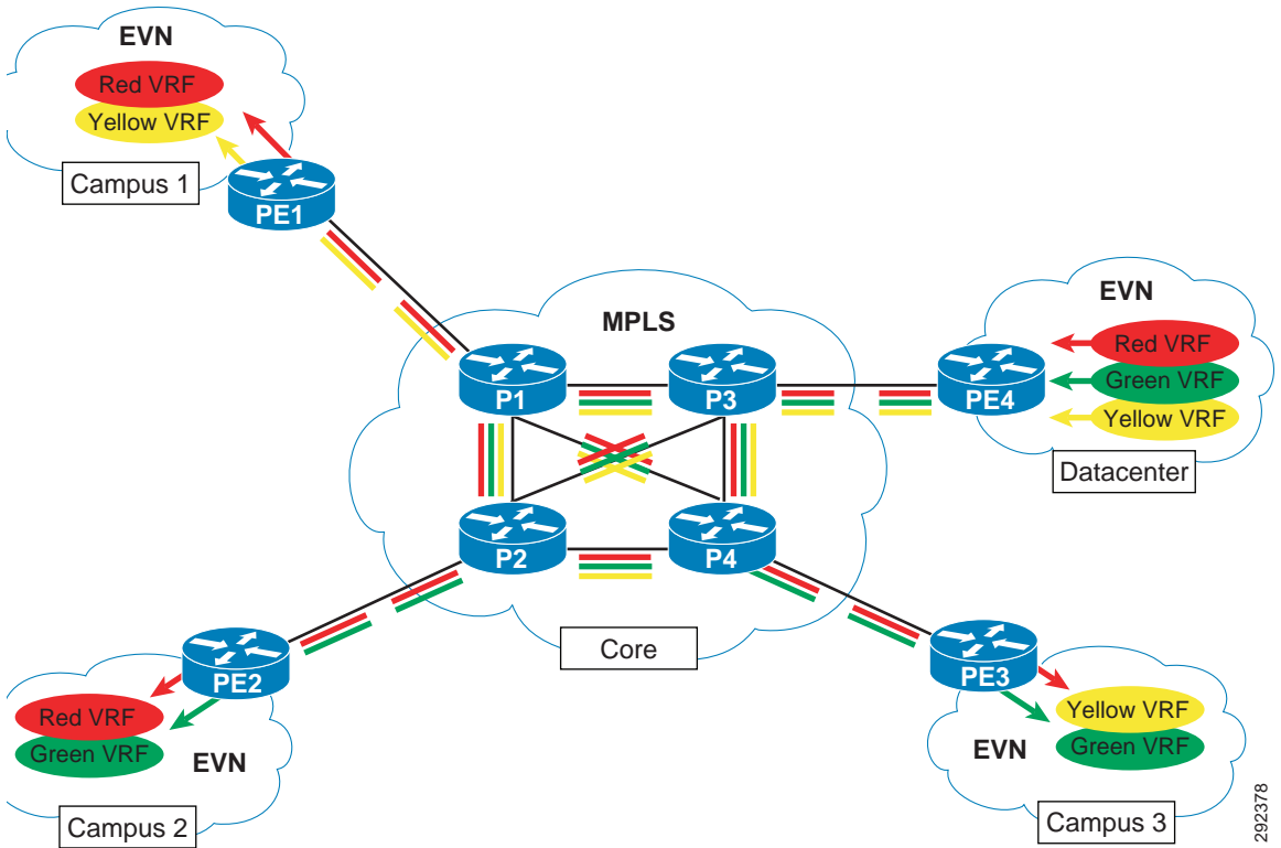
Figure 2 Campus Virtualization Using EVN Interconnected with MPLS Core
