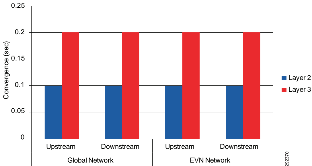
Figure 20 Supervisor Failure HA Analysis
