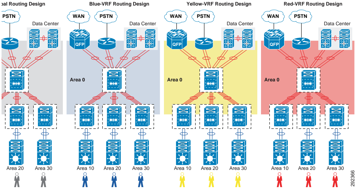
Figure 14 EVN OSPF Routing Design
