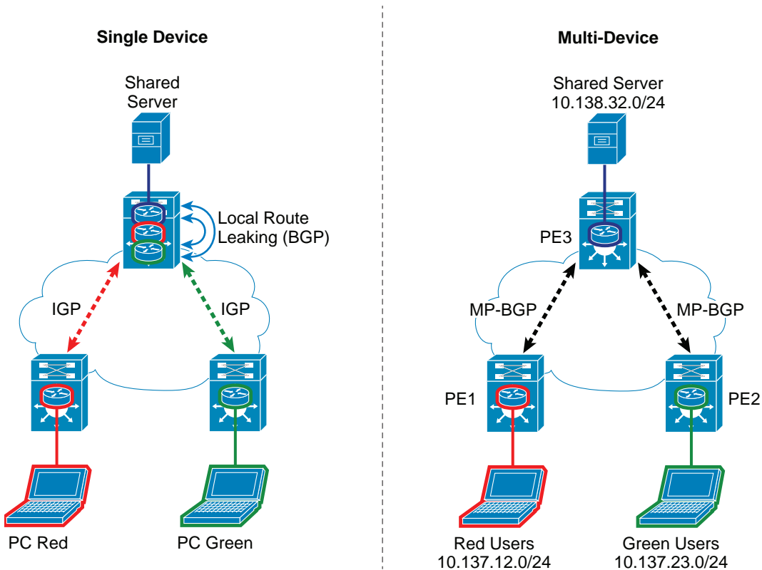
Figure 11 Route Leaking on a Single Device or Multiple Devices
