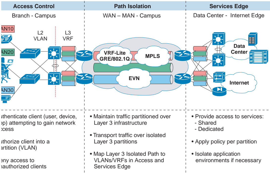
Figure 6 Network Virtualization Architecture
