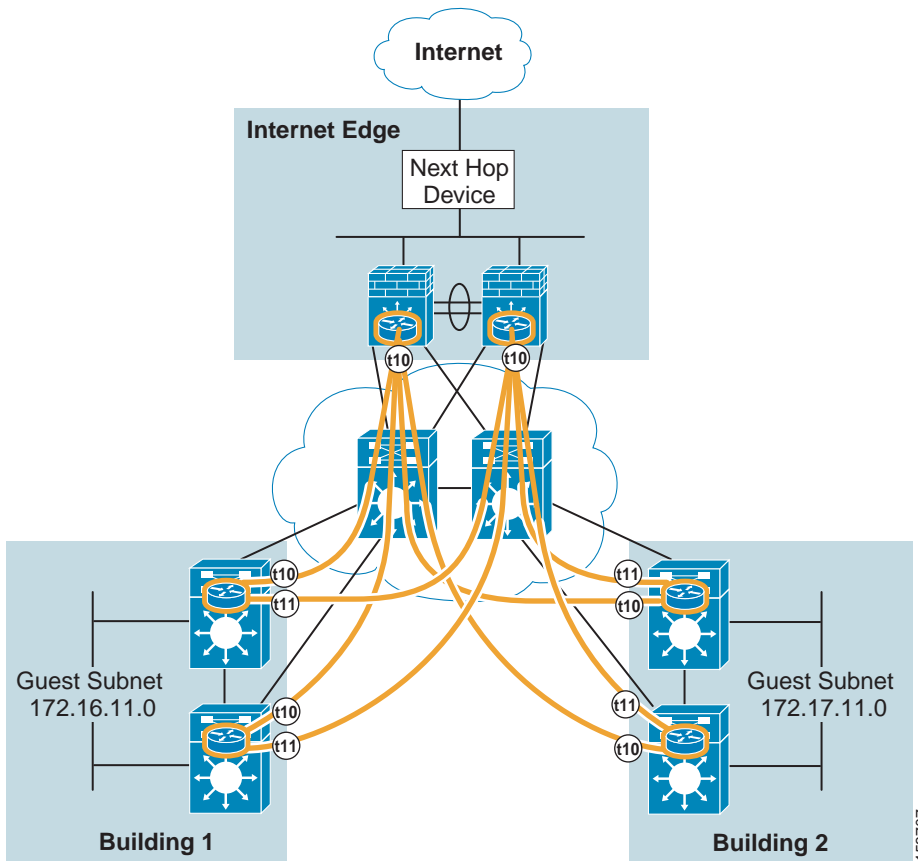
Figure 10 VRF-Lite Used in Conjunction with mGRE at the Hub Routers
