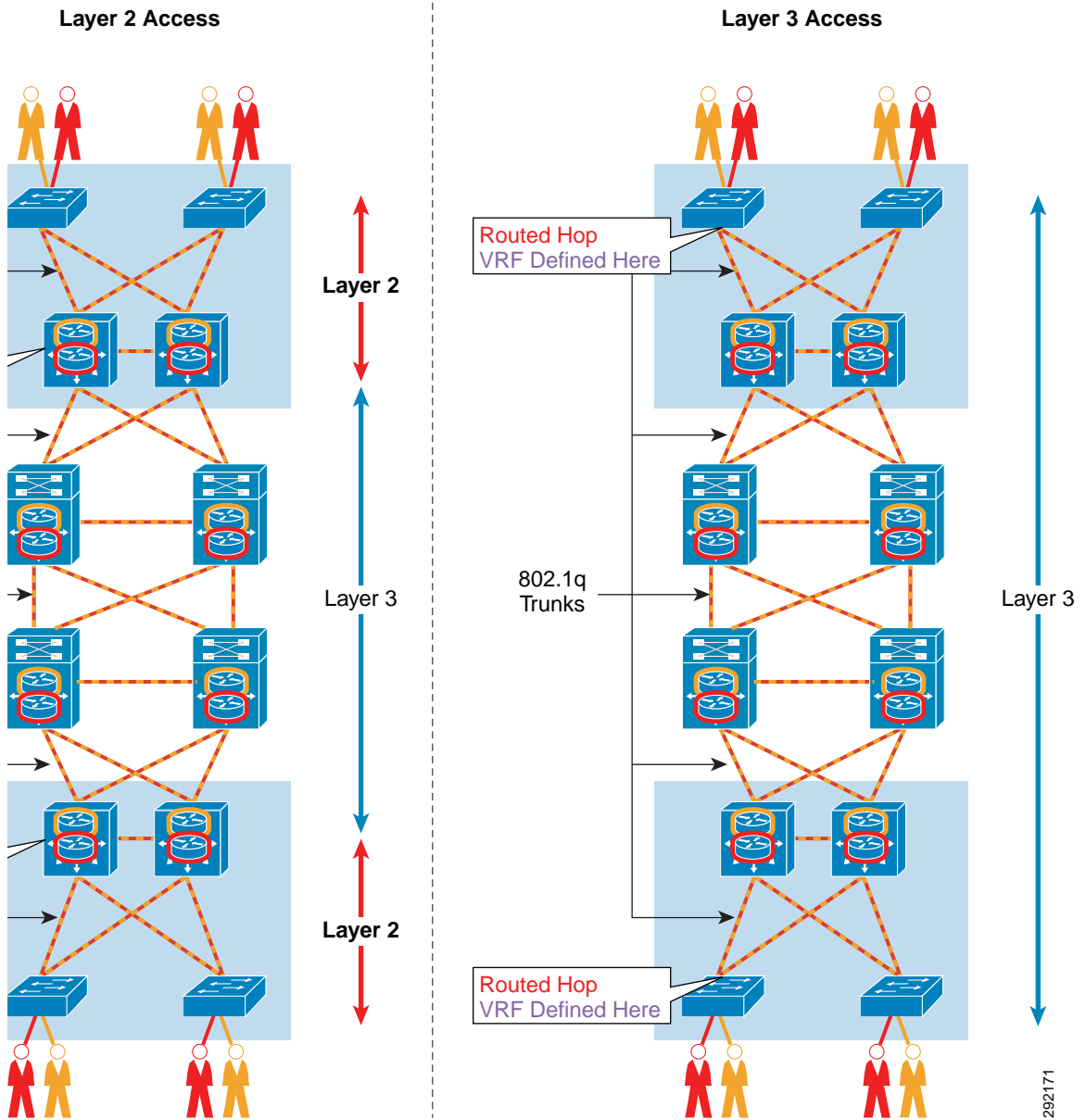
Figure 7 VRF Definition
