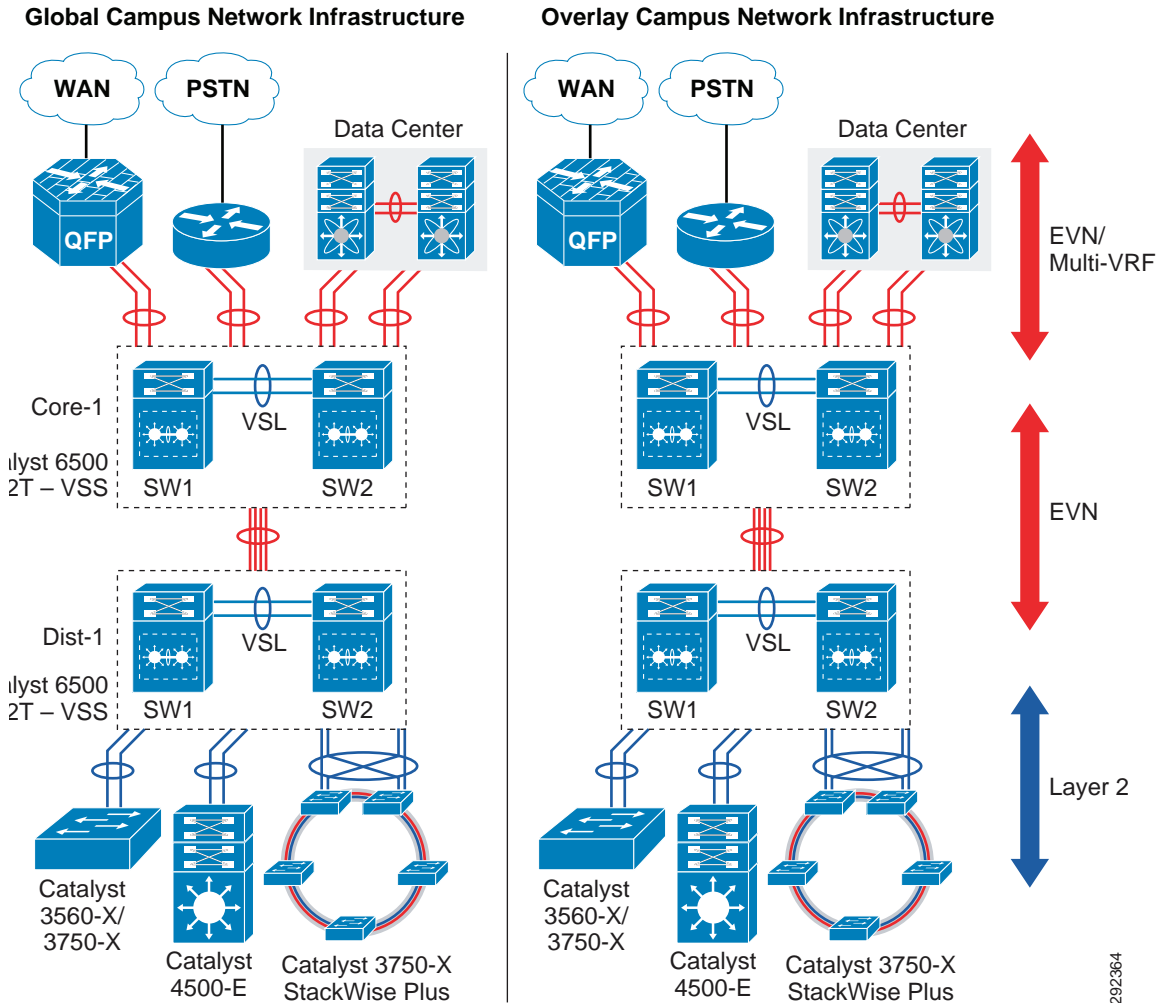
Figure 12 Hop-by-Hop Path Isolation with EVN in Campus
