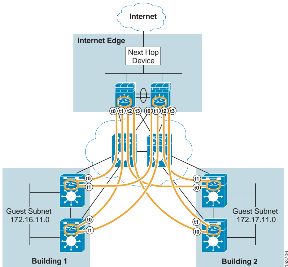
Figure 10 depicts the same campus network except a mGRE Tunnel is defined at hub device.
