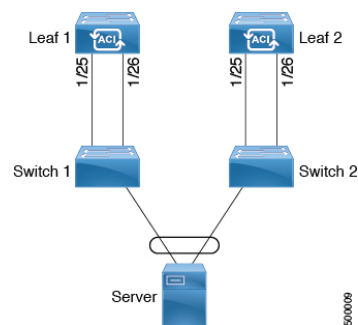
Figure 6: Virtual port channel configuration
