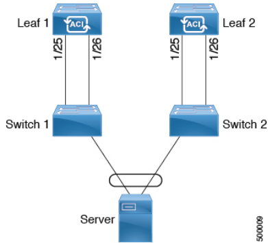
Figure 10: Switch Virtual Port Channel Configuration
