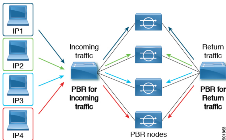
Figure 17: Symmetric PBR
