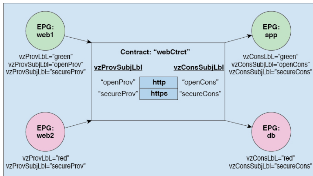
Figure 16: Contracts Determine EPG to EPG Communications
