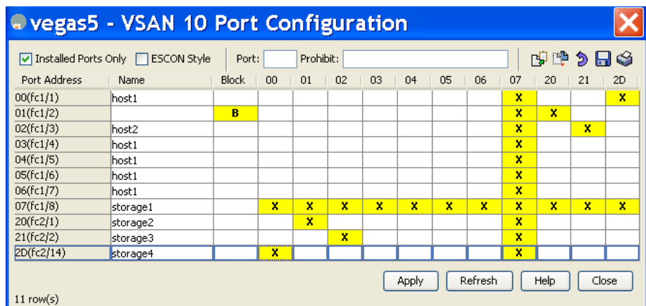
Figure 35-14 FICON Port Configuration Dialog Box
