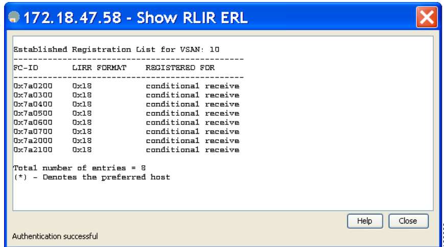
Figure 35-16 Show RLIR ERL Dialog Box
