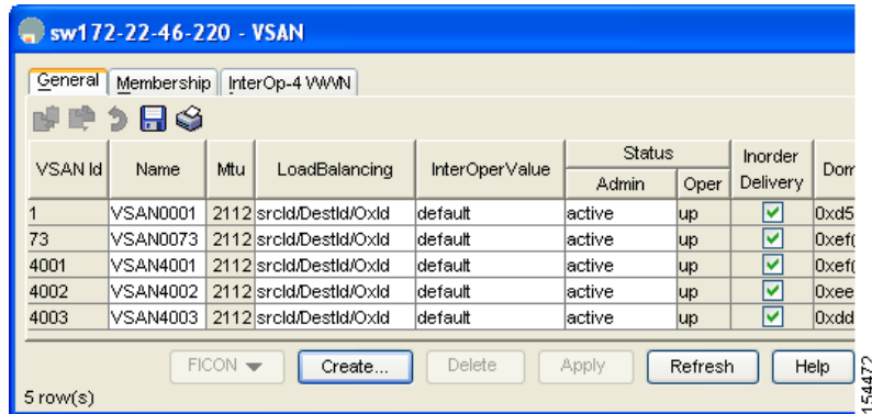
Figure 35-9 VSAN Dialog Box in Device Manager
