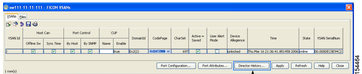
Figure 35-11 FICON VSANs Tab in Device Manager
